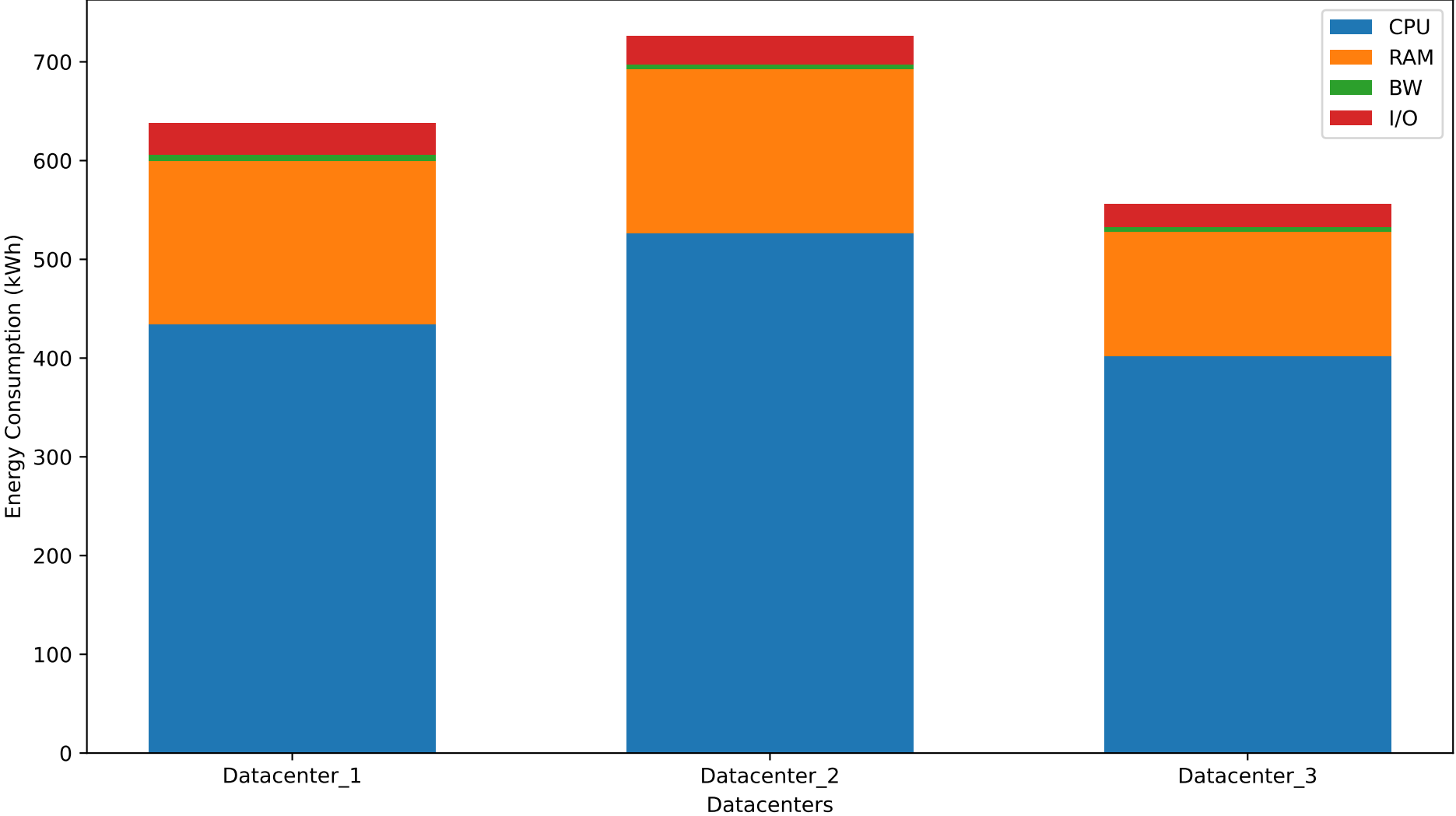
Baseline Scenario: Power Consumption per Datacenter (Stacked by Component)
